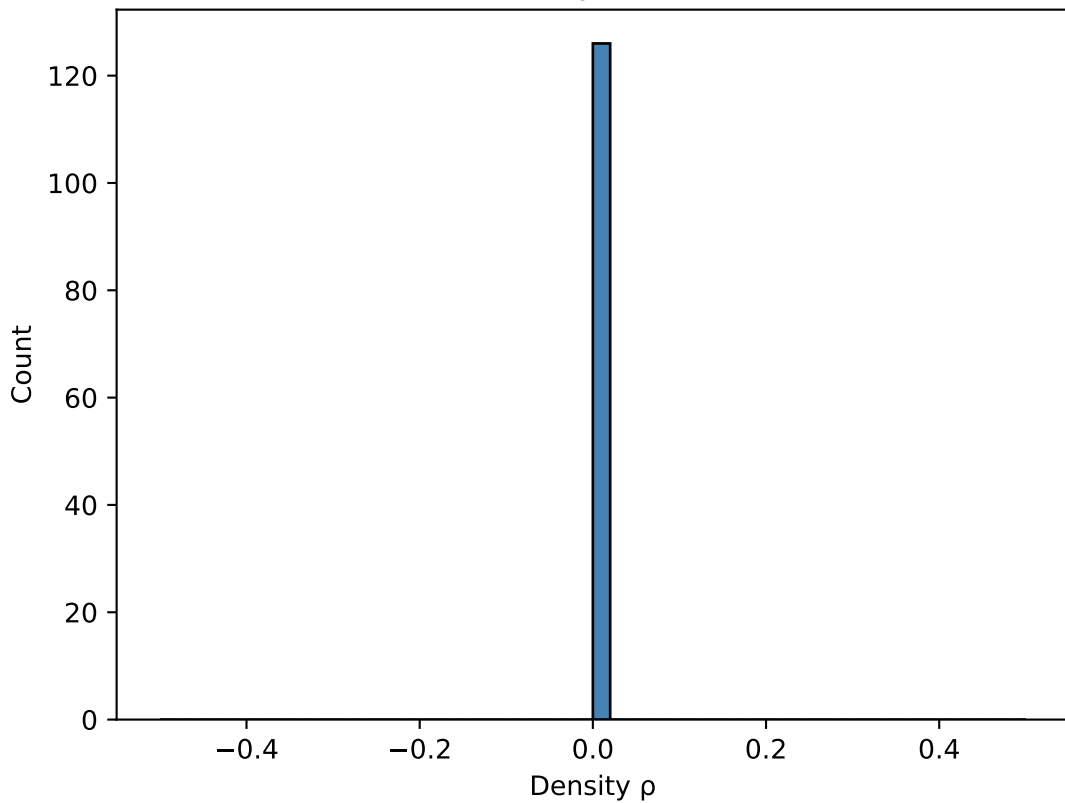
Final density distribution
