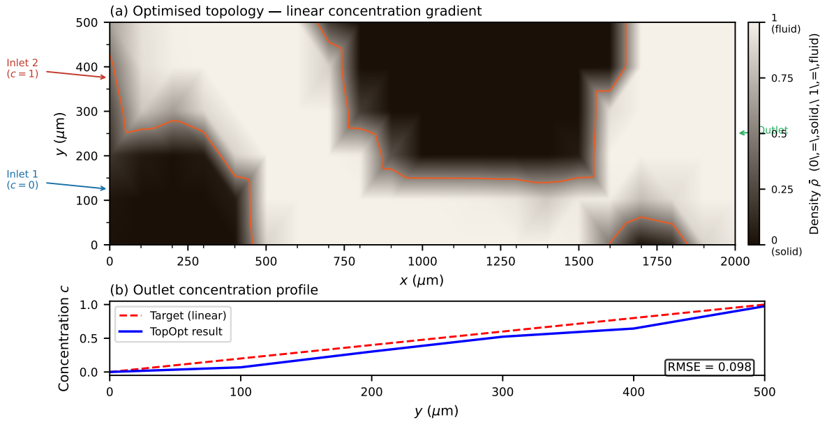
Figure 4: Optimised material distribution for the linear gradient target. Bright regions ( \bar{\rho} \approx 1 ) are fluid; dark regions ( \bar{\rho} \approx 0 ) are solid.
