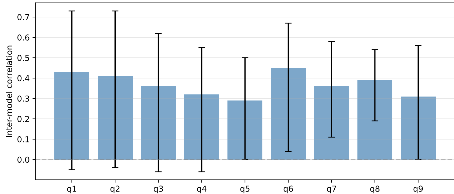
Inter-model correlations per criterion (focus set) error bars: min/max range
