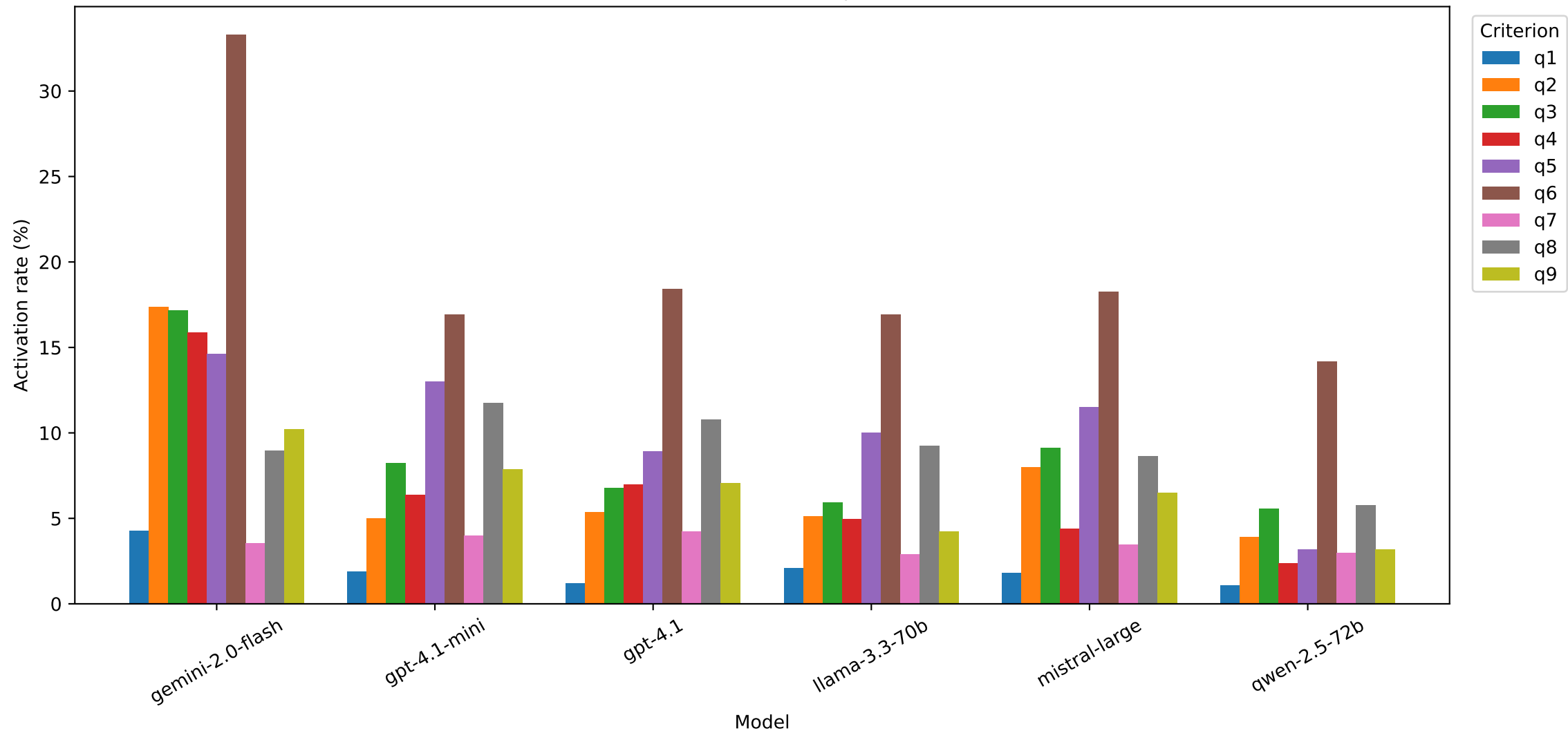
Per-model activation rates per criterion
