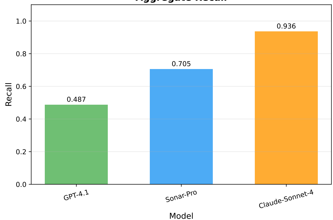
Aggregate Recall
