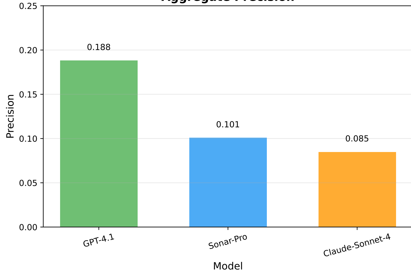
Aggregate Precision
