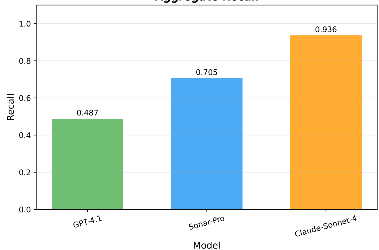
Aggregate Recall
