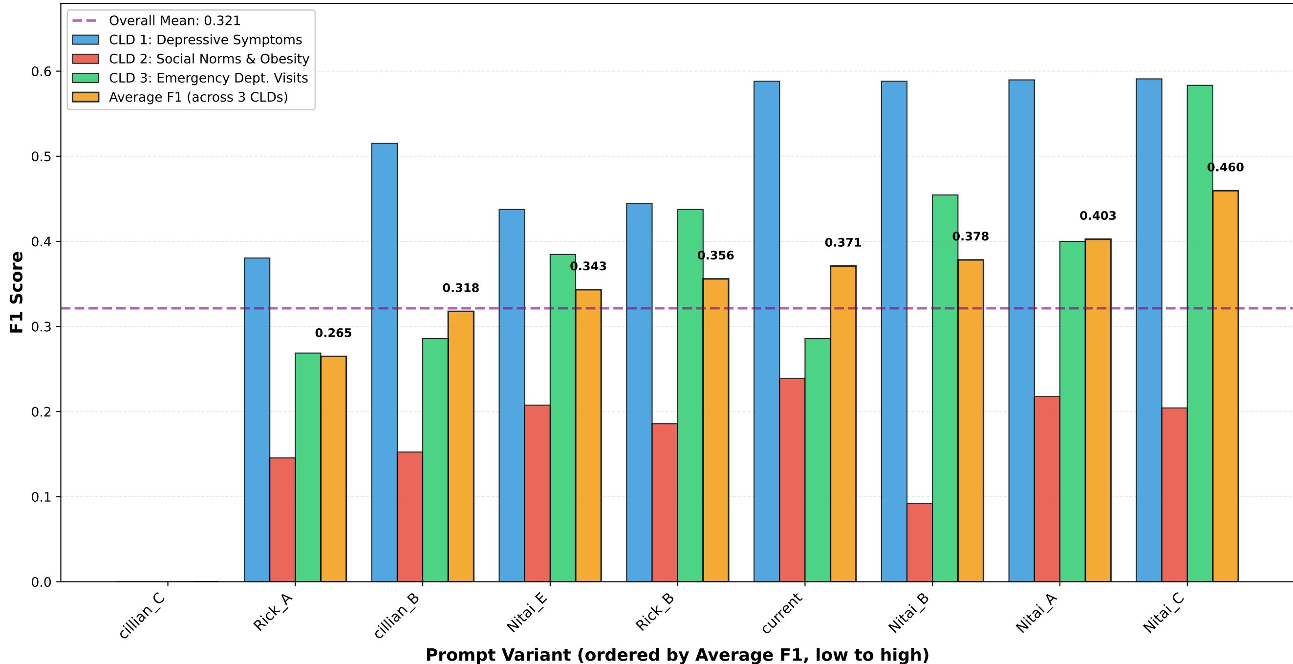
F1 Score Performance: Individual CLDs and Average Prompts Ordered by Average F1 Performance
