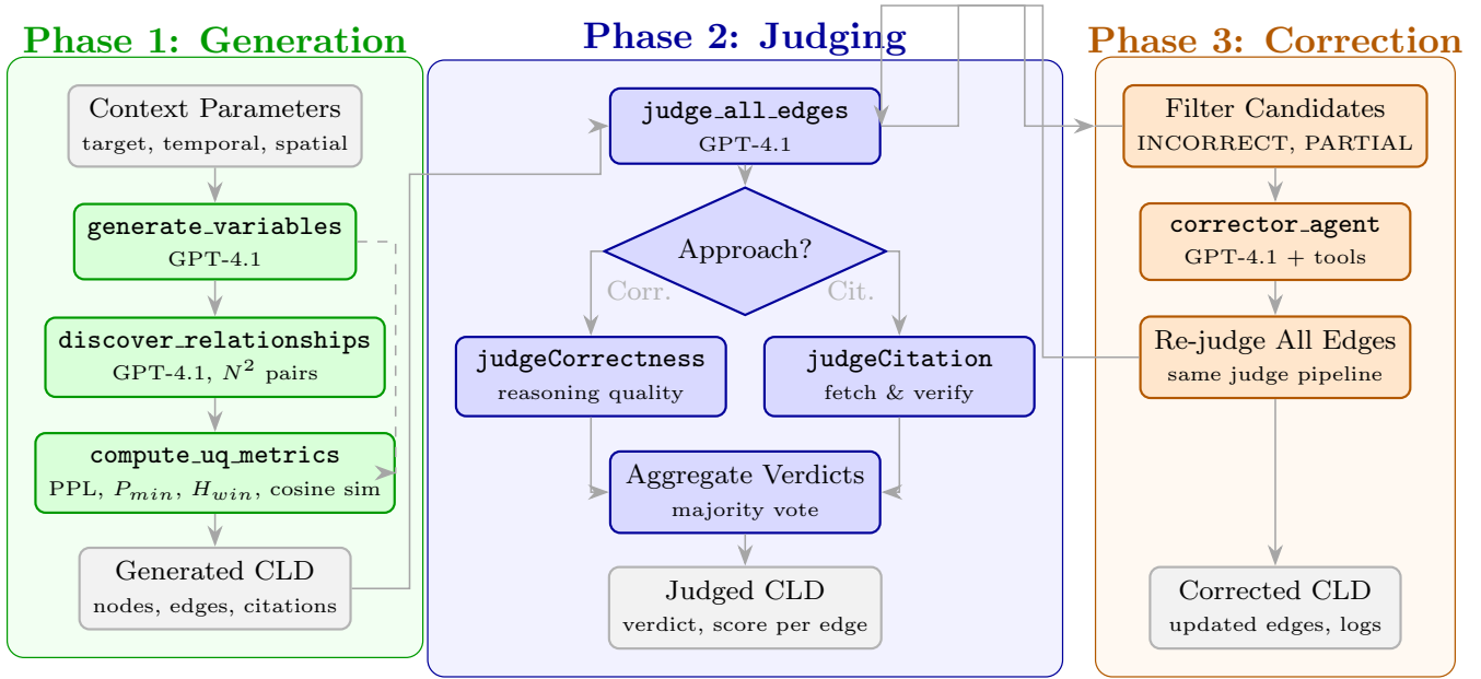
Figure 1: Complete CLD pipeline showing three phases: Generation (green) creates variables and edges with UQ metrics capture, Judging (blue) evaluates edge quality via correctness or citation-based approaches, and Correction (orange) applies LLM-guided fixes to flagged edges with optional re-judging.
