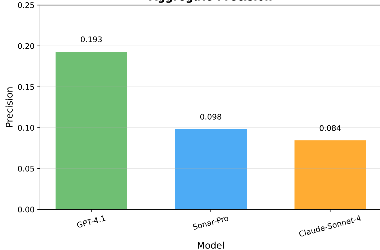
Aggregate Precision
