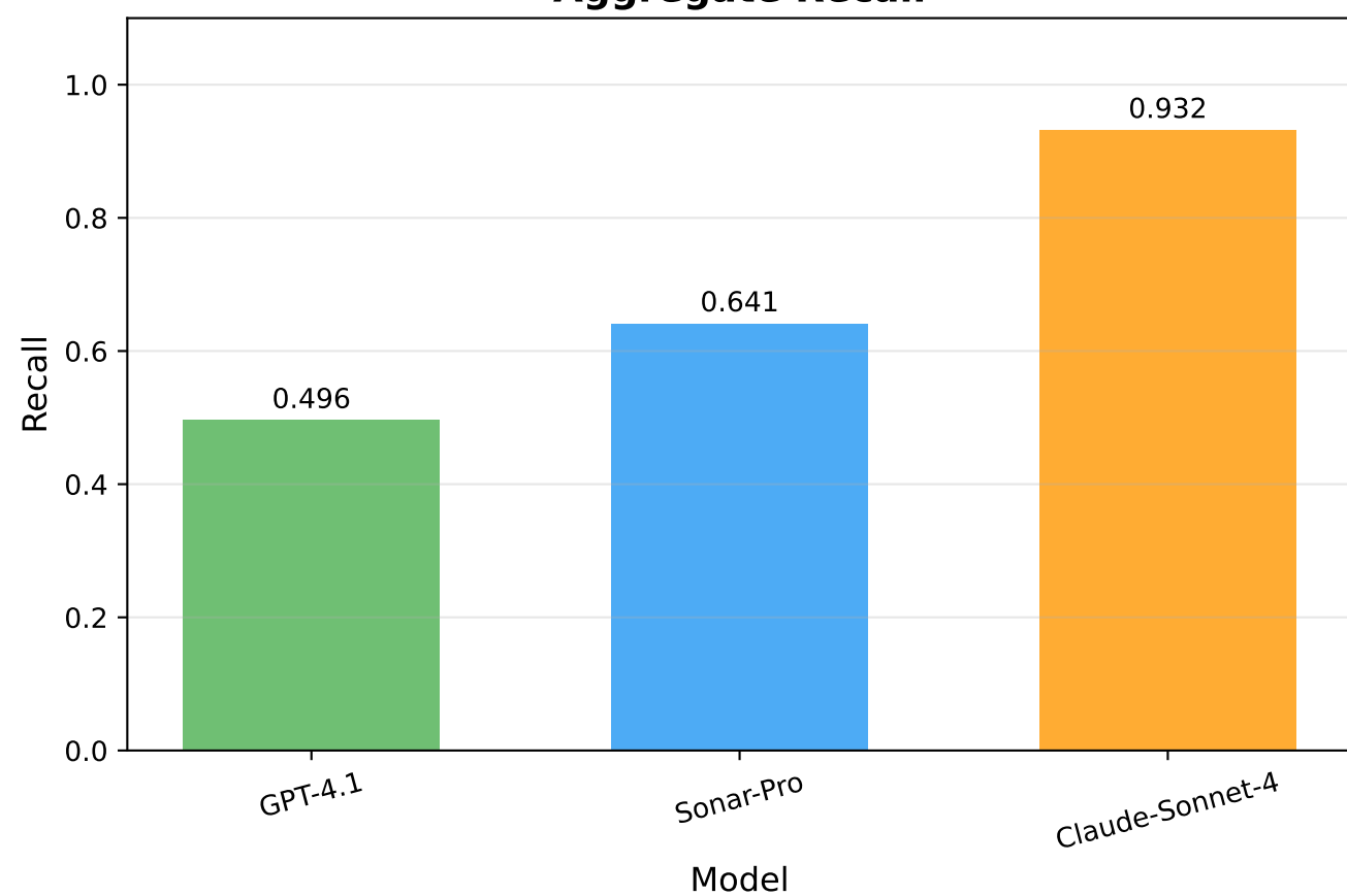
Aggregate Recall
