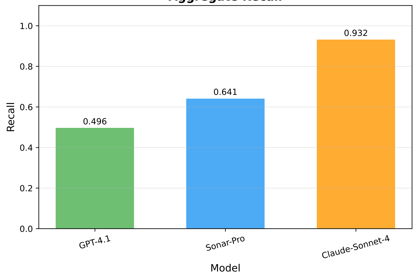
Aggregate Recall
