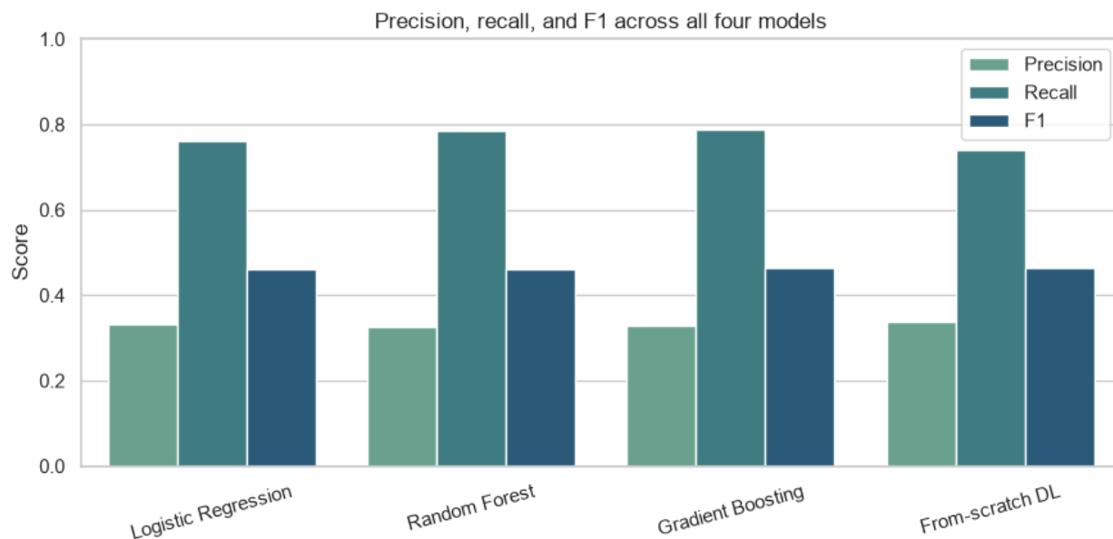
Figure 5: Precision, recall, and F1 across all four diabetes models.
