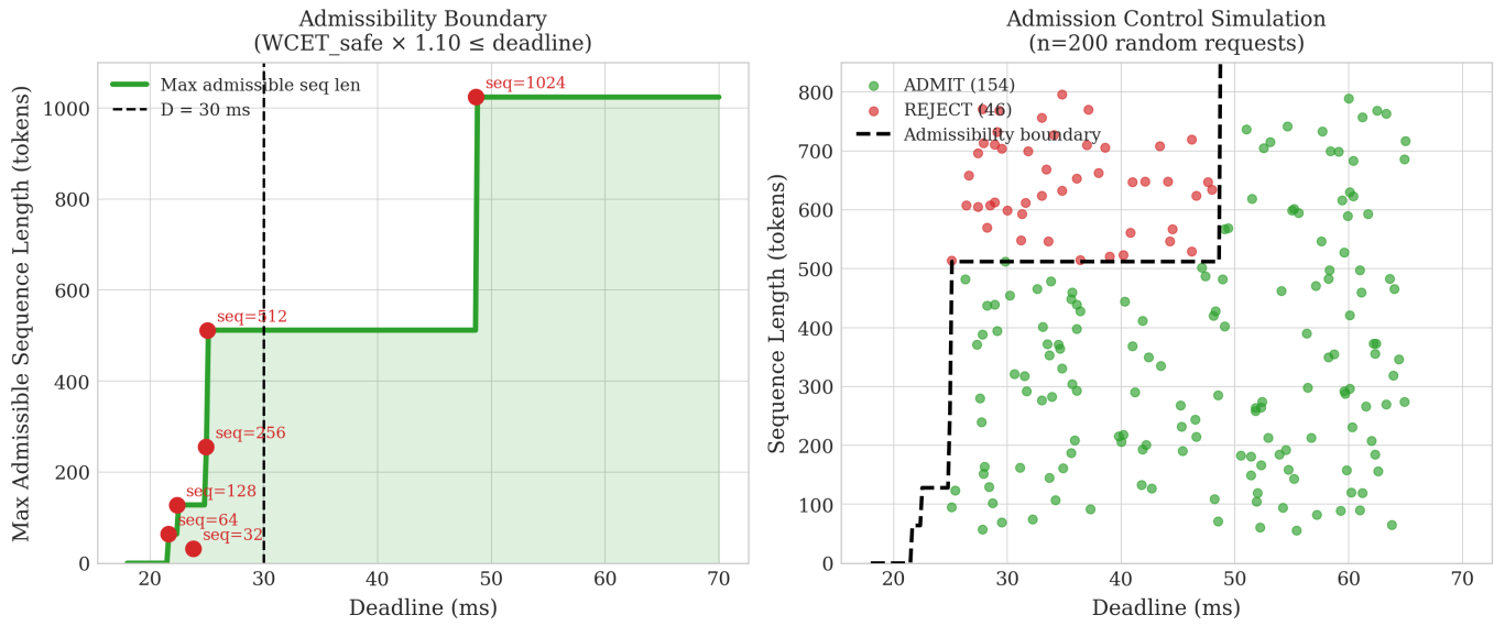
Fig. 11. Admission control analysis. Left : ADMIT/REJECT boundary with WCET annotations. Right : simulation of 200 random requests (seq Uniform[50,800], deadline Uniform[25,65] ms).
