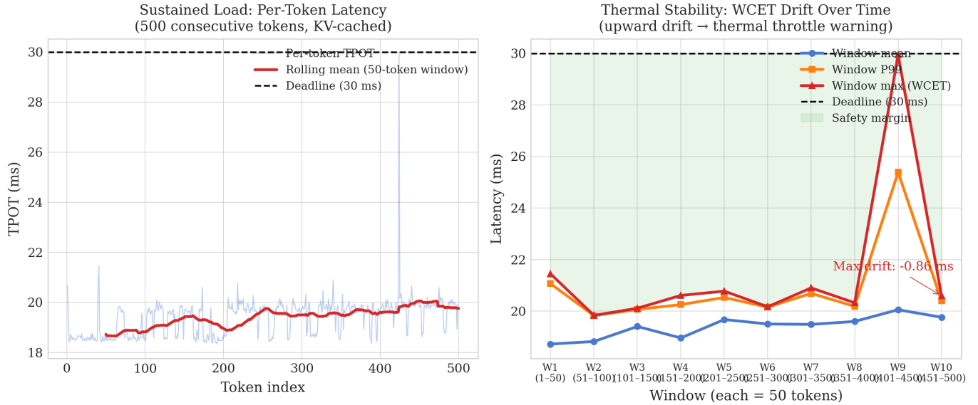
Fig. 8. Thermal stability profile (500 consecutive tokens, KV-cached router, RTX 6000 Ada). Left : raw TPOT time series with 50-token rolling mean. Right : per-window summary with drift annotation. No systematic upward trend is observed; isolated spikes return to baseline within the next window.
