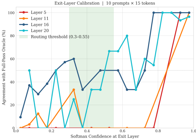
Fig. 2. Exit-layer ablation (L5, L11, L16, L20 vs. full-pass oracle). Agreement rate vs. confidence threshold. Layer 16 is the inflection point where agreement jumps from 2.7% (L11) to 32.0% and high-confidence agreement reaches 64.7%.
