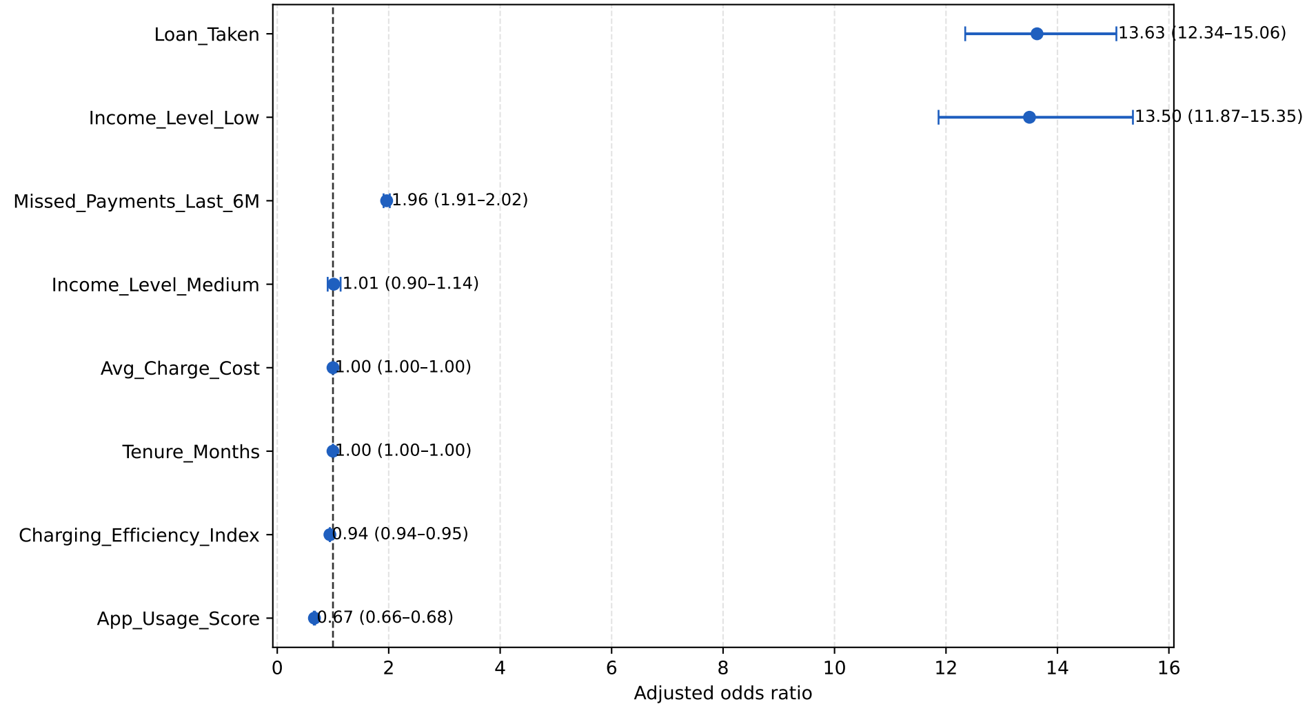
Figure 2. Financial predictors of high default risk
