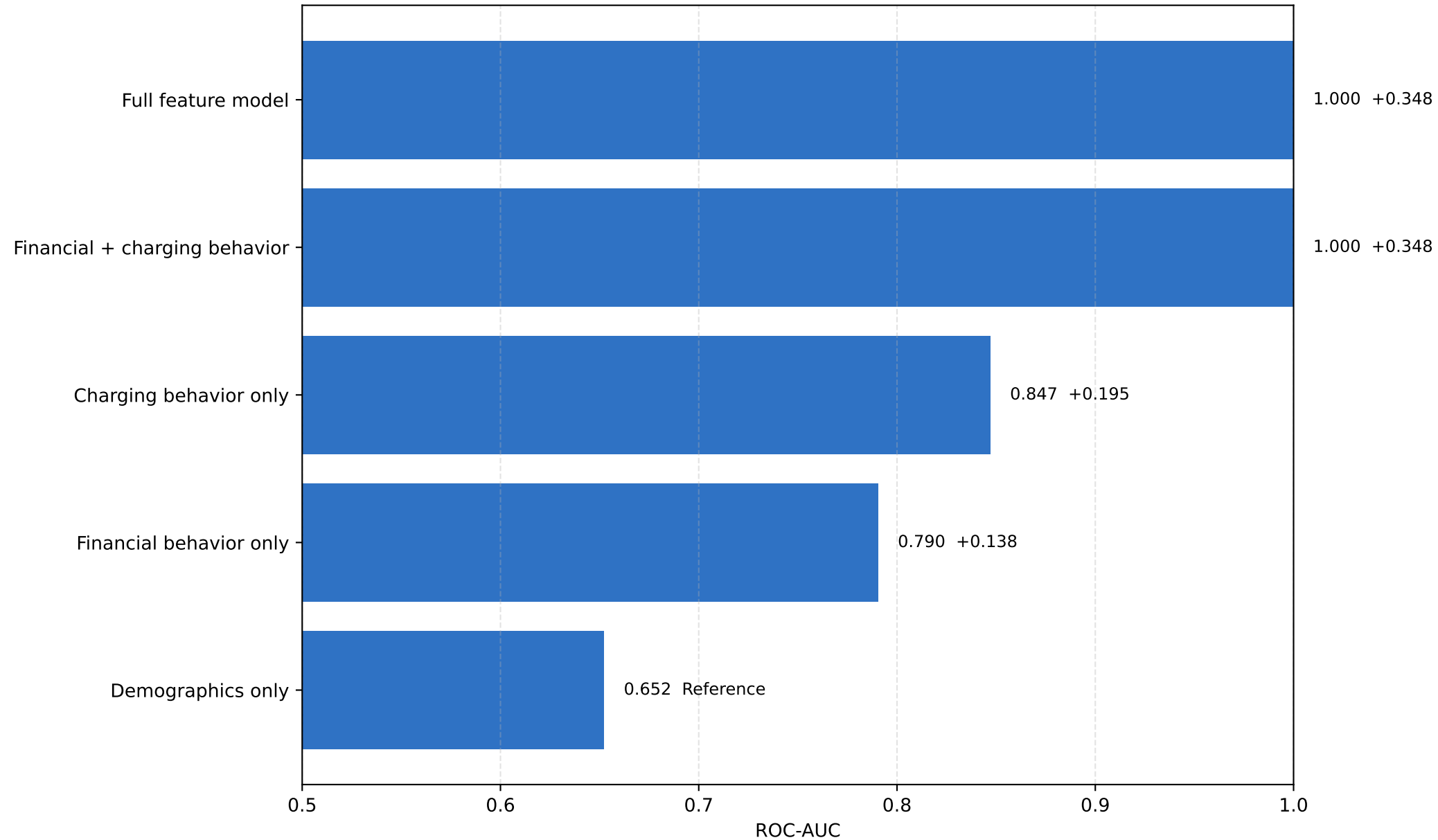
Figure 3. Incremental gain after adding charging-behavior features
