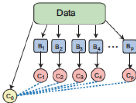
A) Bootstrapping Stability: scheme 1
