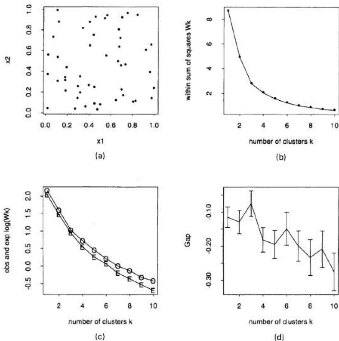
Fig. 2. Results for the uniform data example: (a) data; (b) within sum of squares function W_k ; (c) functions \log(W_k) (O) and E_n^*(\log(W_k)) (E); (d) gap curve
