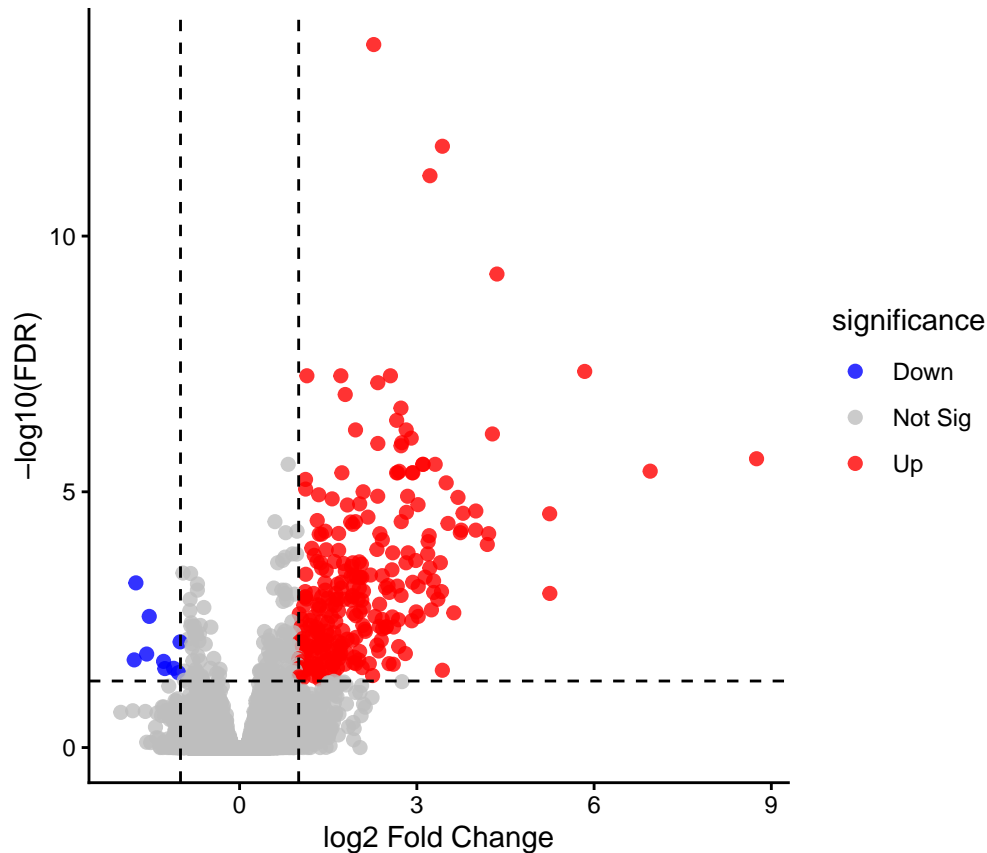
EdgeR Volcano Plot 20 days (PCI vs Sham)
