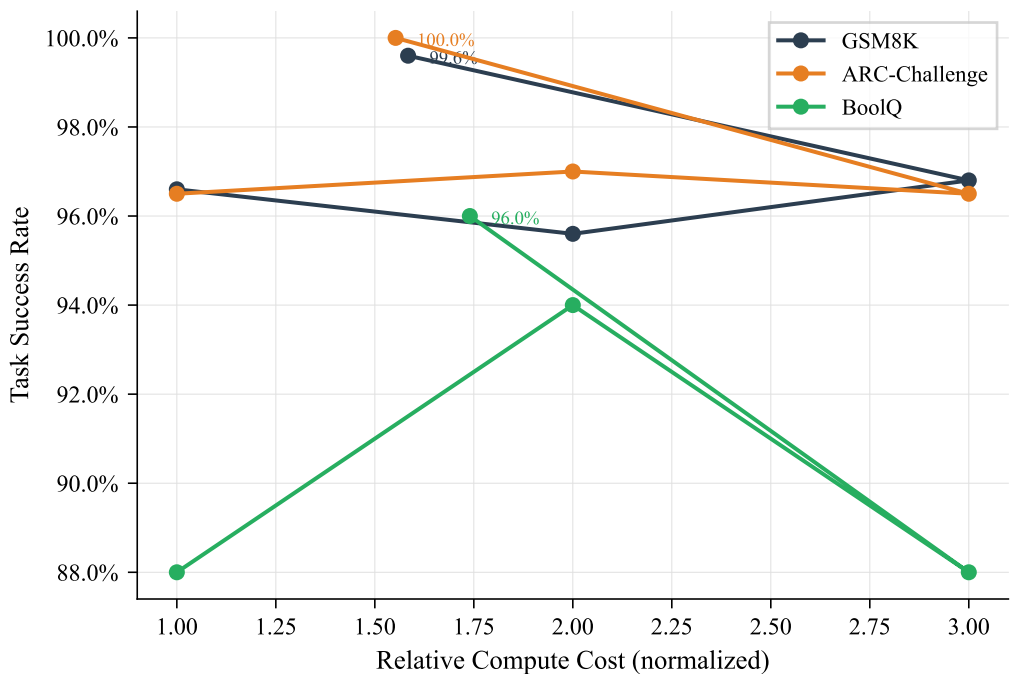
Figure 7: Accuracy–Compute Efficiency Frontier
