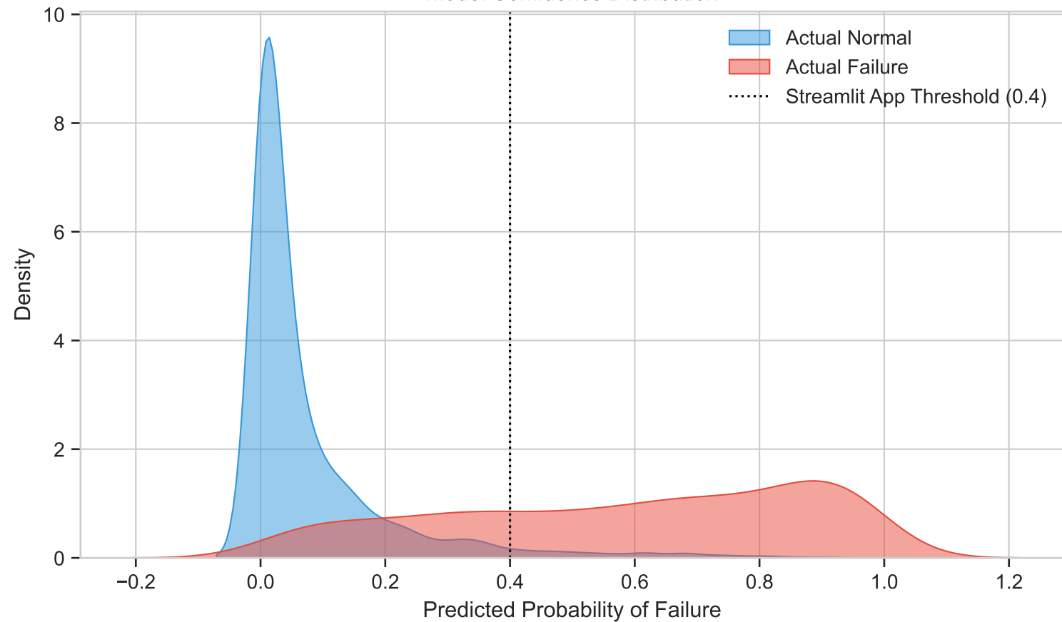
Model Confidence Distribution
