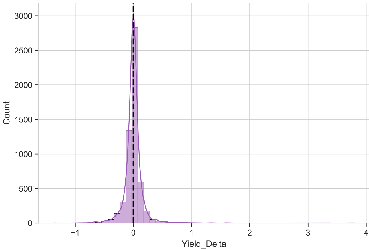
Residual Distribution (Prediction Errors)
