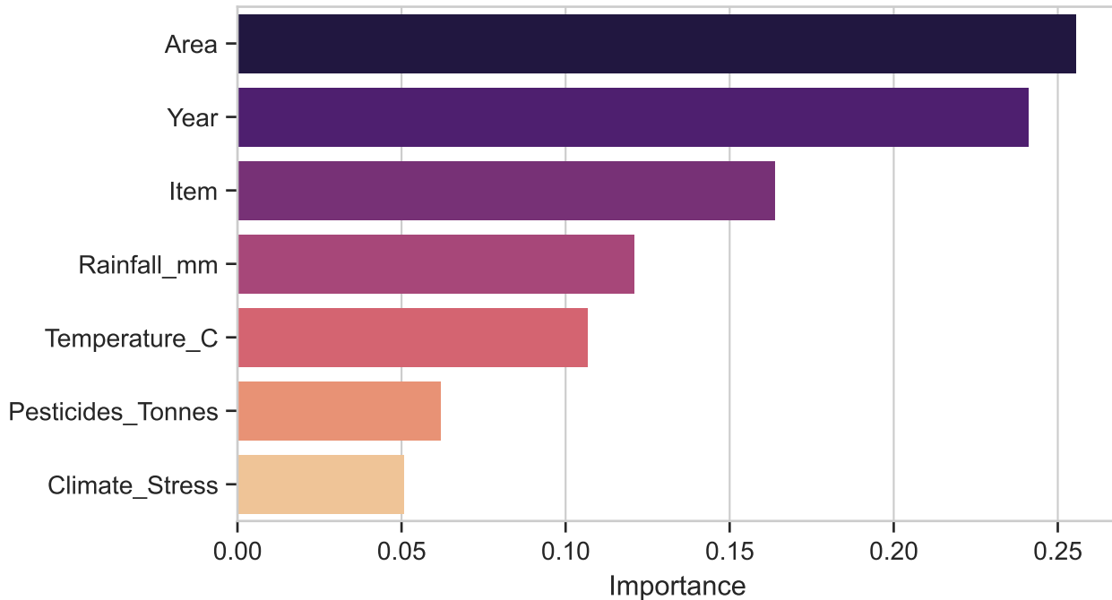
Regression Factors (Feature Importance)
