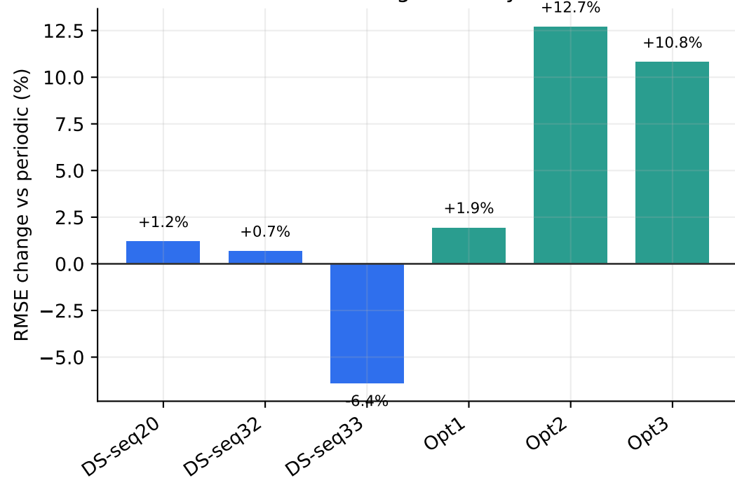
Tracking accuracy
