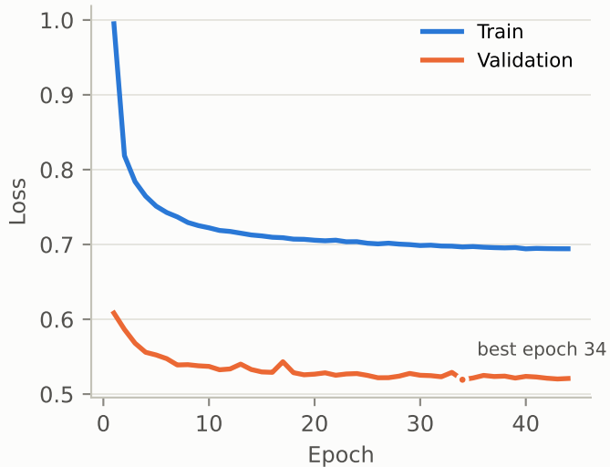
Cross-entropy loss
