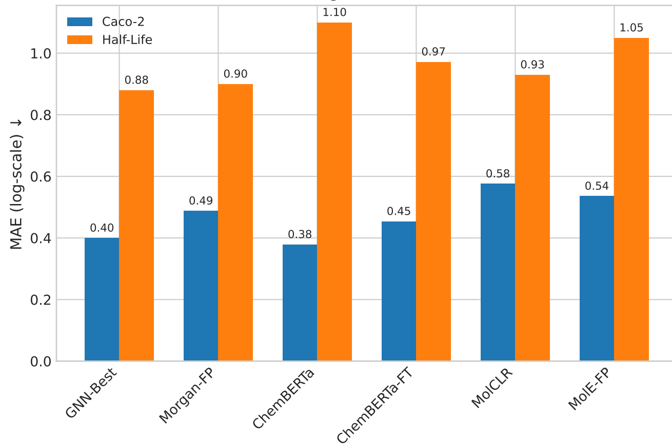
(a) ADME Regression Performance
