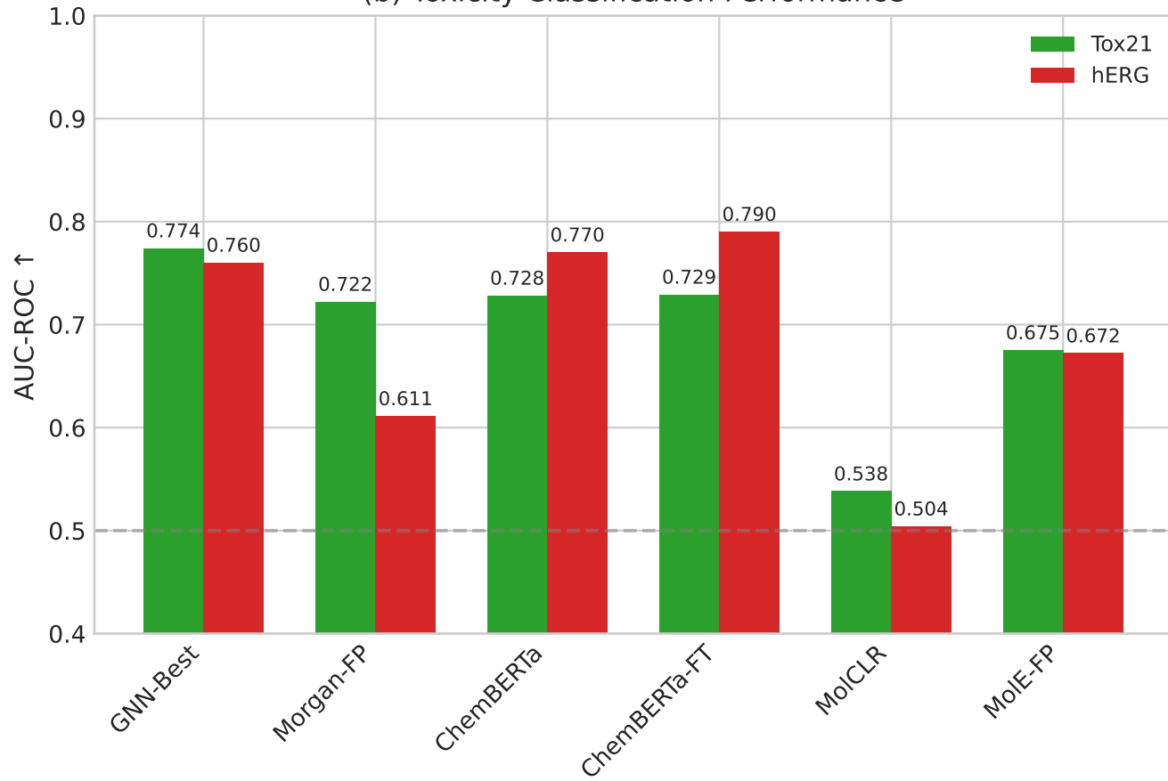
(b) Toxicity Classification Performance
