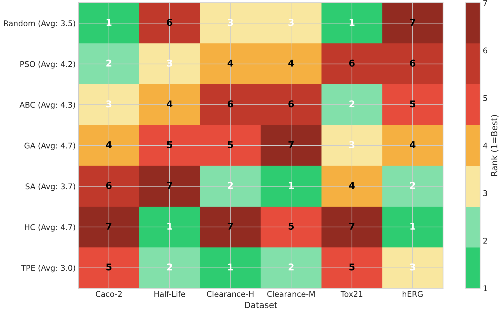
HPO Algorithm Ranking Across Datasets
