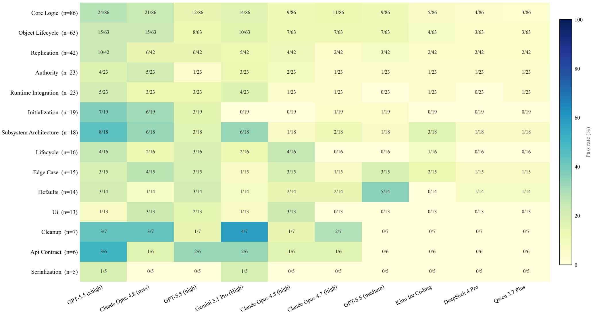
Pass rate by requirement category (top 14)
