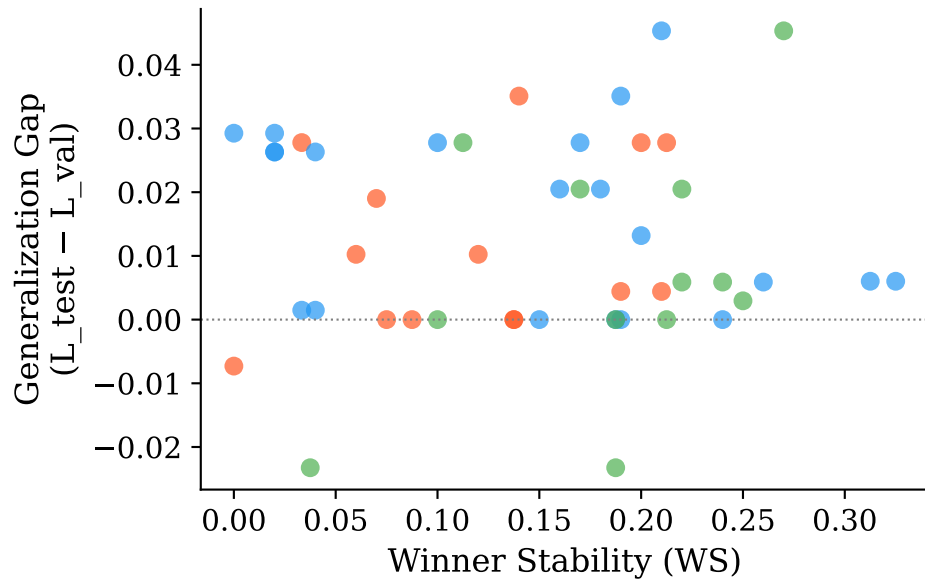
Winner Stability vs. Generalization Gap Spearman r=-0.01 , p=0.922 ( n=47 )
