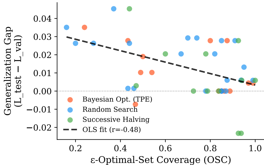
OSC vs. Generalization Gap Spearman r=-0.39 , p=0.006 ( n=47 )
