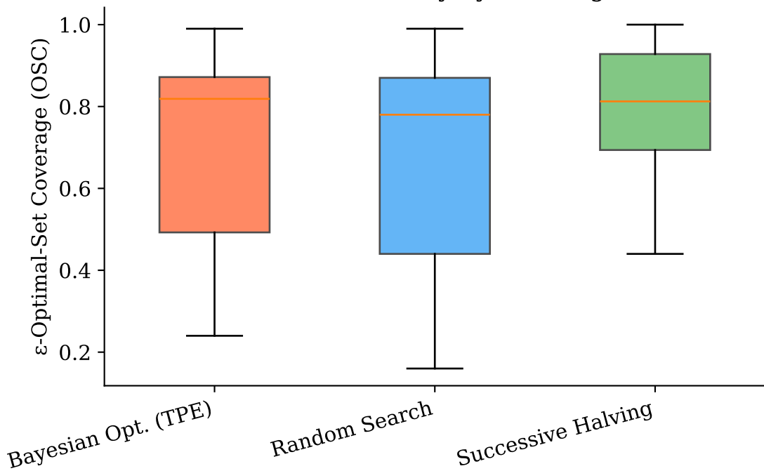
Selection Uncertainty by HPO Algorithm
