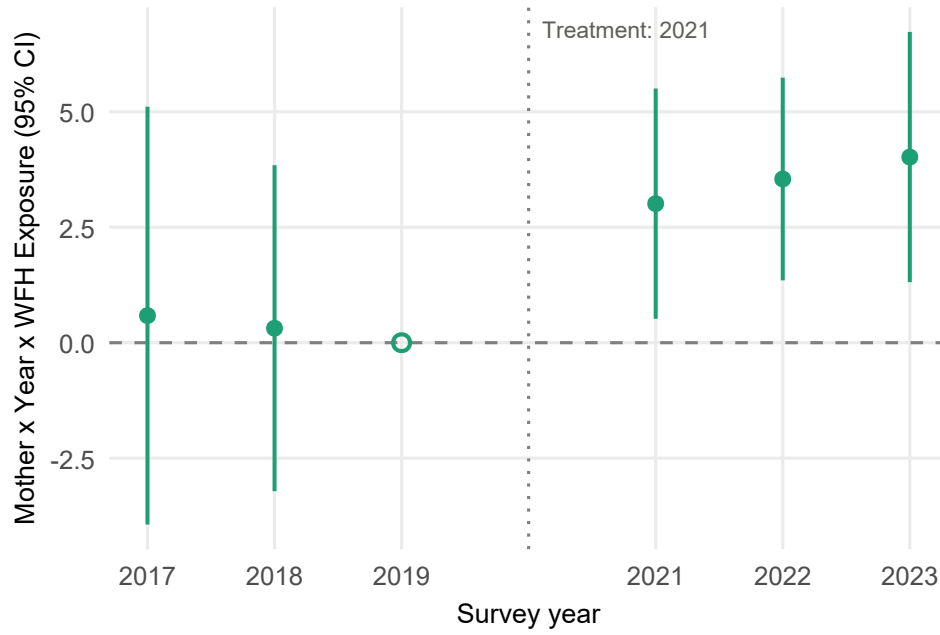
Figure 4: Event study for the triple difference: \text{Mother} \times \text{year} \times \text{WFH\_Exposure} interactions for weekly hours, reference year 2019
