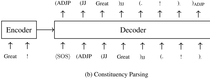
Figure 6.6: Illustration of tree linearization on either the encoder or decoder side. For tree-to-string machine translation, the encoder takes a sequential representation of an input parse tree, and the decoder outputs the corresponding translation. For parsing, the encoder takes a sentence, and the decoder outputs the corresponding syntax tree.
