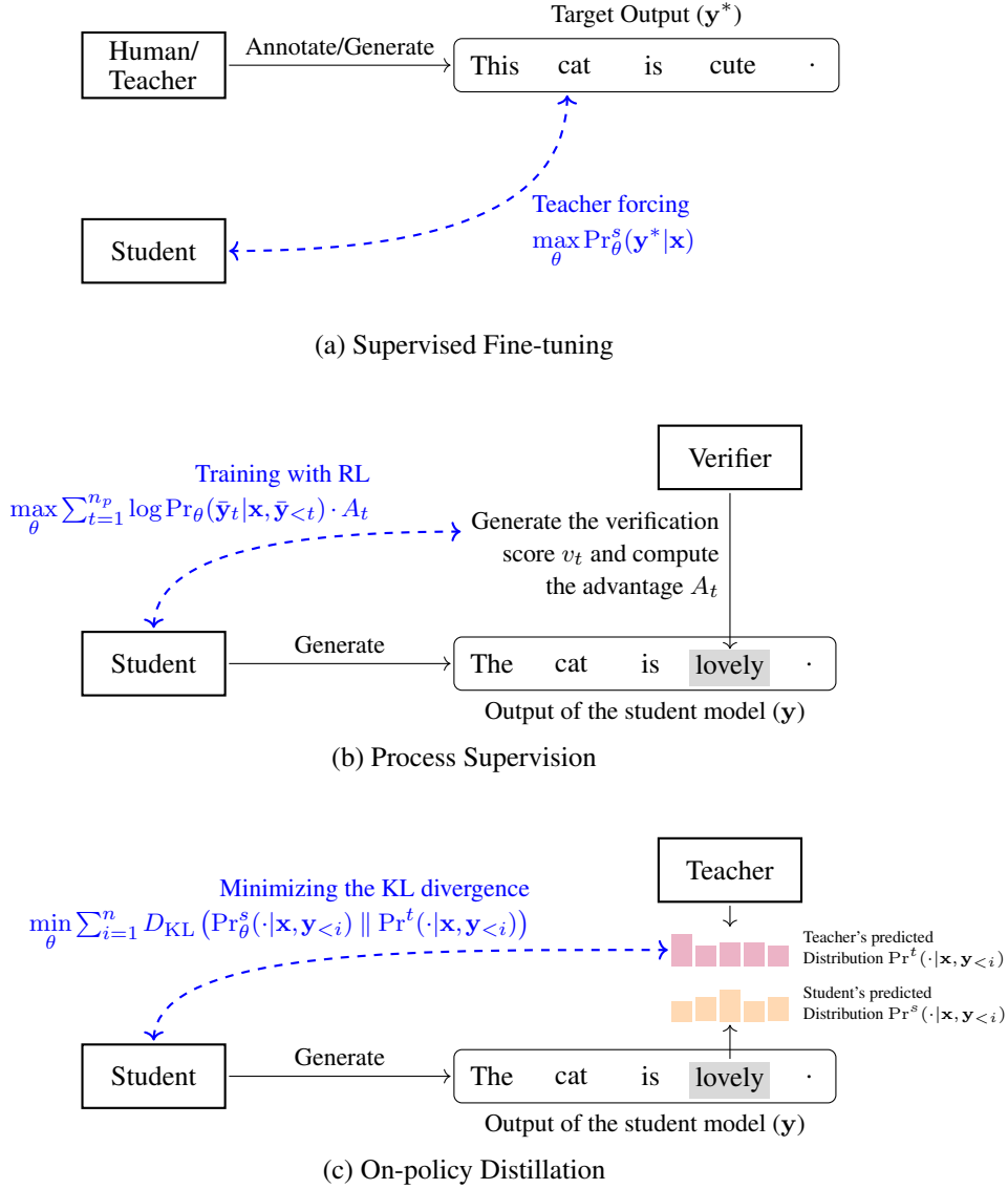
Figure 12.2: Comparison of supervised fine-tuning, process supervision, and on-policy distillation methods. In supervised fine-tuning (a), the student model is trained off-policy to maximize the likelihood of golden target outputs provided by a human or a teacher model. In process supervision (b), the student model generates its own reasoning path, and a verifier evaluates these self-generated steps to compute advantages. In on-policy distillation (c), the student also generates its own path, but instead of scalar rewards, a teacher model provides a dense, token-level probability distribution at each step. The student is updated by minimizing the KL divergence between its own predicted distribution and the teacher's distribution.
