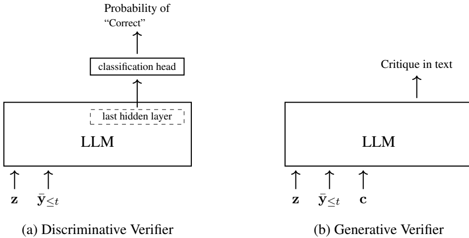
Figure 12.1: Comparison between discriminative and generative verification approaches. Subfigure (a) shows a discriminative verifier which attaches a classification head to the last hidden layer of the LLM to output a numerical probability of correctness. Subfigure (b) shows a generative verifier that prompts the LLM with the query \mathbf{z} , reasoning history \bar{\mathbf{y}}_{\leq t} , and an instruction \mathbf{c} to generate a natural language critique instead of a scalar value.
