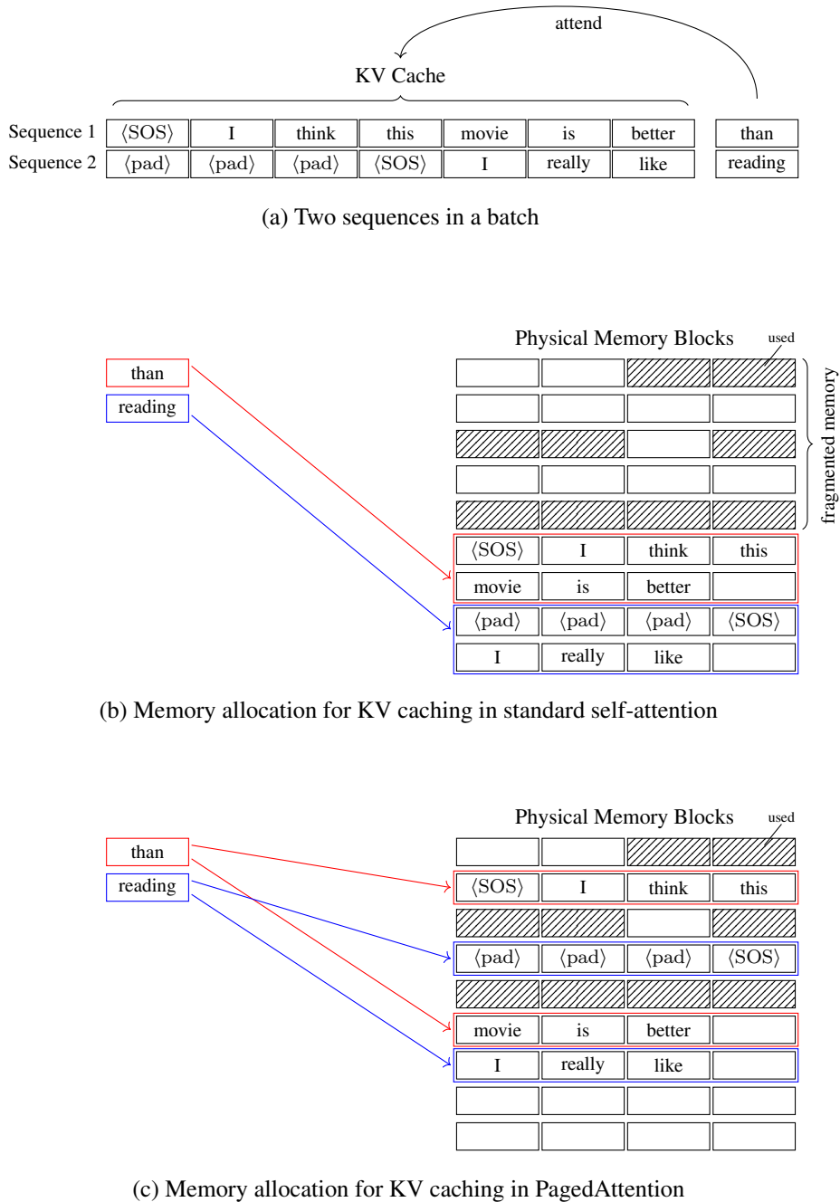
Figure 11.12: Illustration of memory allocation in PagedAttention. There are two sequences in the batch, as illustrated in sub-figure (a). Since the memory is fragmented, the KV cache is stored in a large unused block of memory in standard self-attention (see sub-figure (b)), but the fragmented memory is not used. By contrast, in PagedAttention (see sub-figure (c)), the KV cache is divided into smaller blocks and thus fits into fragmented memory.
