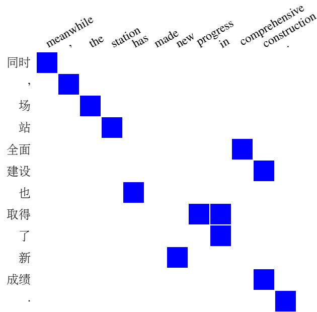
(a) Heat map of word alignments
