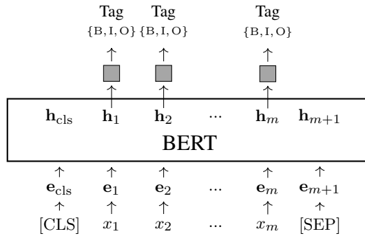
Figure 7.11: BERT-based sequence labeling for named entity recognition. Here \{B, I, O\} is the tag set of NER.
