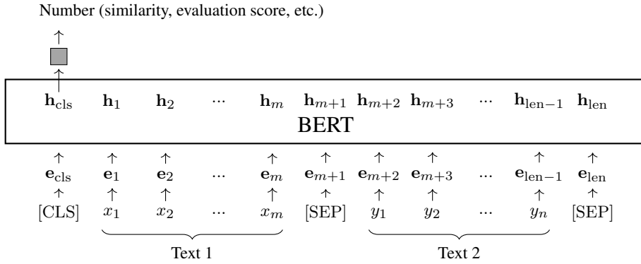
Figure 7.10: BERT-based regression for a pair of texts.
