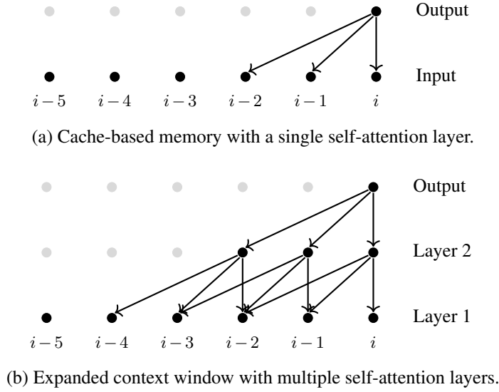
Figure 6.15: Cache-based memory mechanism in Transformer models.
