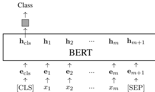
Figure 7.8: BERT-based classification for a single text. Here the gray box denotes the prediction network.
