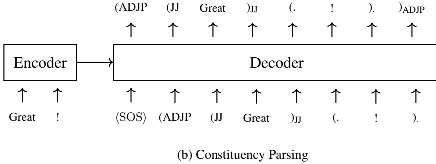
Figure 6.6: Illustration of tree linearization on either the encoder or the decoder side. For tree-to-string machine translation, the encoder takes a sequential representation of an input parse tree, and the decoder outputs the corresponding translation. For parsing, the encoder takes a sentence, and the decoder outputs the corresponding syntax tree.
