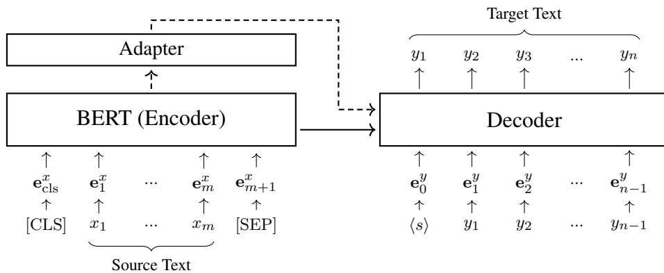
Figure 7.13: Using BERT as the encoder in an encoder-decoder model. Here x_1 \cdots x_m denotes the source sequence, y_1 \cdots y_n denotes the target sequence, e_1^x \cdots e_m^x denotes the embedding sequence of x_1 \cdots x_m , and e_1^y \cdots e_n^y denotes the embedding sequence of y_1 \cdots y_n . The adapter, which is optional, maps the output of the BERT model to the form that is better suited to the decoder.
