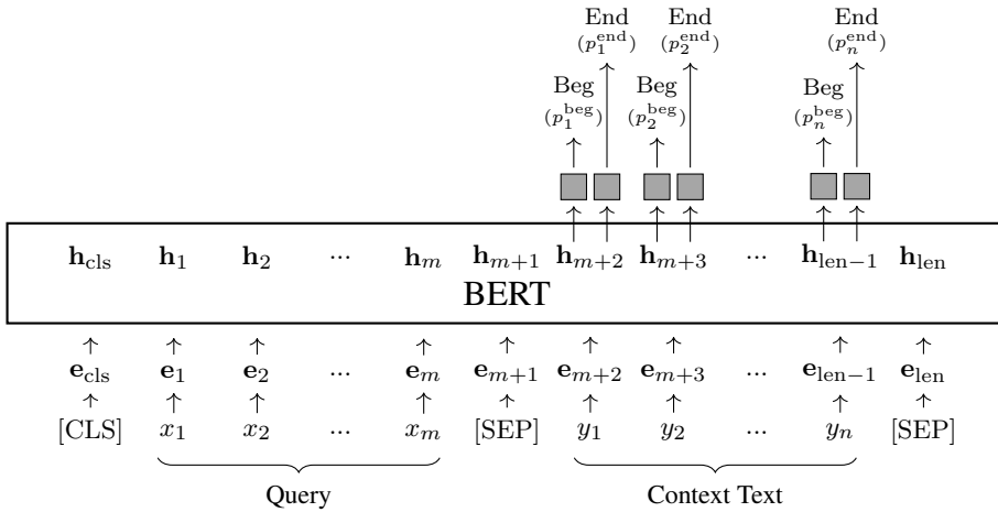
Figure 7.12: BERT-based span prediction for reading comprehension.
