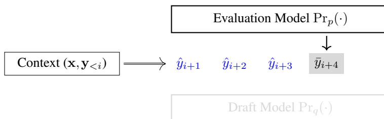
Figure 11.7: Illustration of one step of speculative decoding. The goal is to predict as many next tokens as possible using the draft model. There are four sub-steps. Given the context, we first use the draft model to predict the next \tau tokens. Then, we evaluate these predictions in parallel using the verification model. Next, we determine the maximum number of predicted tokens that can be accepted. Finally, we use the evaluation model to predict a new token following these accepted tokens.
