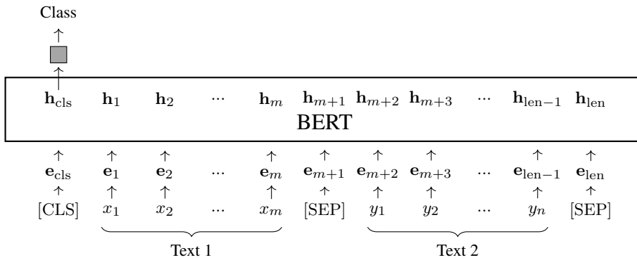
Figure 7.9: BERT-based classification for a pair of texts. Here, \text{len} = n + m + 2 .
