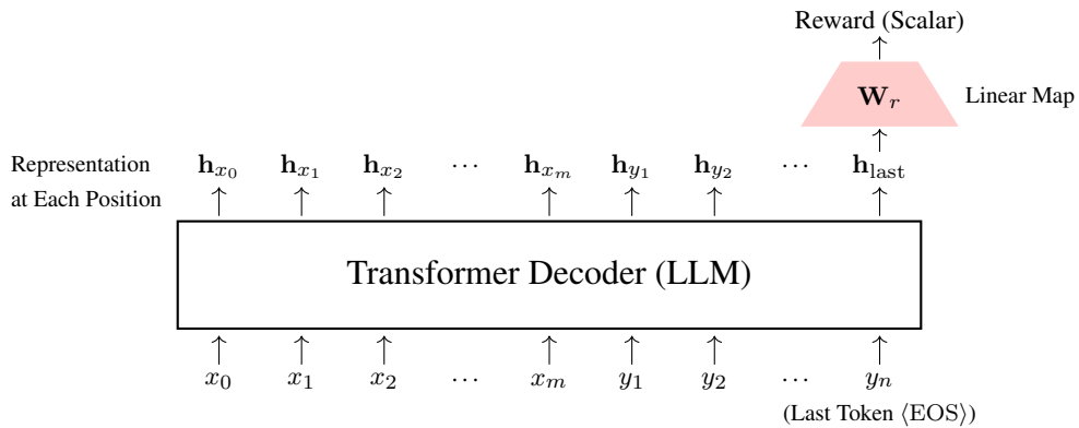
Figure 10.8: Architecture of a Transformer-based reward model. The main component of this model is still an LLM. We use the Transformer decoder as the sequence representation model. We take the representation at the last position of the decoder as the representation of the entire sequence [\mathbf{x}, \mathbf{y}] . We then map this representation to a scalar through a linear transformation, which serves as the reward score for [\mathbf{x}, \mathbf{y}] .
