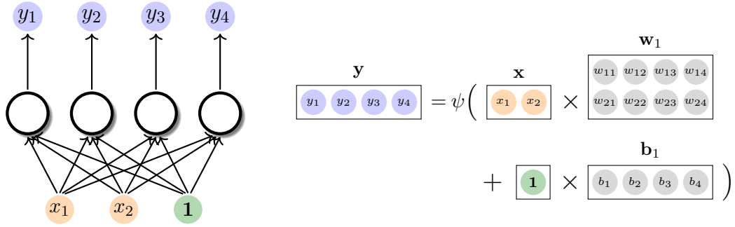
Figure 2.2: A single-layer perceptron involving four neurons. All these neurons receive information from the input variables \{x_1, x_2\} . The perceptron describes a process where 1) we first transform the input vector of variables by an affine transformation f(\mathbf{x}) = \mathbf{x} \cdot \mathbf{w} + \mathbf{b} ; and 2) compute the output by feeding f(\mathbf{x}) into the activation function \psi(\cdot) .
