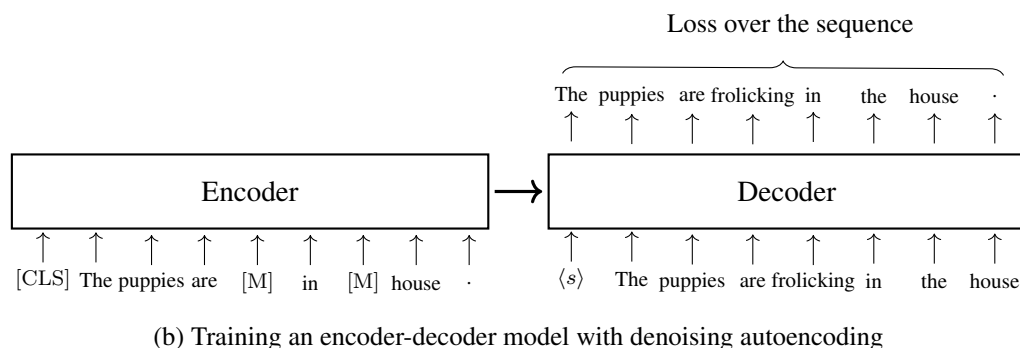
Figure 7.4: Training an encoder-decoder model using BERT-style and denoising autoencoding methods. In both methods, the input to the encoder is a corrupted token sequence where some tokens are masked and replaced with [MASK] (or [M] for short). The decoder predicts these masked tokens, but in different ways. In BERT-style training, the decoder only needs to compute the loss for the masked tokens, while the remaining tokens in the sequence can be simply treated as [MASK] tokens. In denoising autoencoding, the decoder predicts the sequence of all tokens in an autoregressive manner. As a result, the loss is obtained by accumulating the losses of all these tokens, as in standard language modeling.
