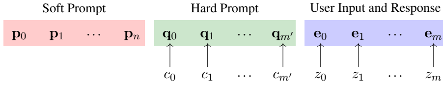
Figure 9.7: A prompt pattern that combines soft prompts, hard prompts, and user input. Here, c_0 \cdots c_{m'} denotes the hard prompt and q_0 \cdots q_{m'} denotes the corresponding embedding sequence.
