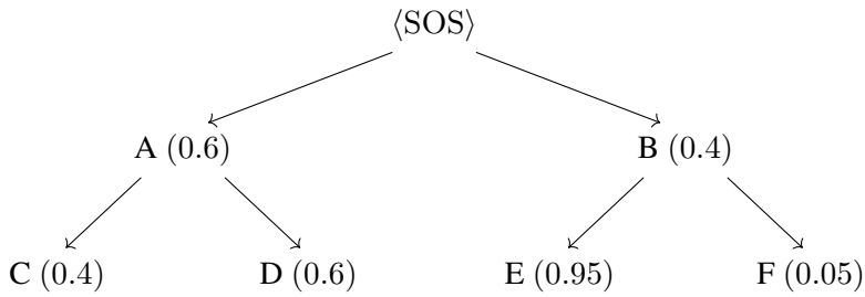
Figure 5.12: Illustration of a simple search tree.
