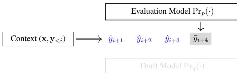
Figure 11.7: Illustration of one step of speculative decoding. The goal is to predict as many next tokens as possible using the draft model. There are four sub-steps. Given the context, we first use the draft model to predict the next \tau tokens. Then, we evaluate these predictions in parallel using the verification model. Next, we determine the maximum number of predicted tokens that can be accepted. Finally, we use the evaluation model to predict a new token following these accepted tokens.
