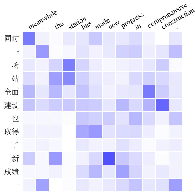
(b) Heat map of attention weights
