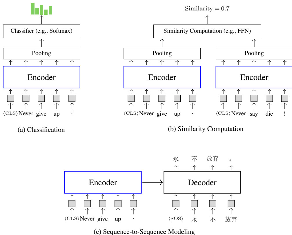
Figure 6.18: Illustration of Integrating Transformer encoders as components of different systems. A common approach is to feed the output of the encoder (with pooling) into a classifier to obtain a sequence classification system. Another way to utilize Transformer encoders is to compute the similarity between two sequences. We use the same encoder to represent the two sequences, and then build a neural network over the two representations to produce a similarity score between them. Furthermore, Transformer encoders can also be used in encoder-decoder systems to model sequence-to-sequence problems.
