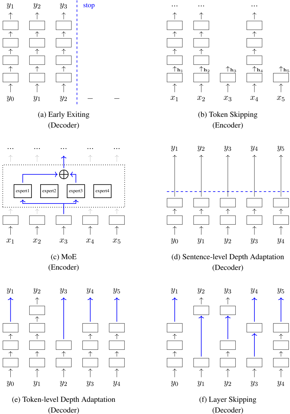
Figure 6.17: Methods of conditional computation, including early exiting, token skipping, MoE, sentence-level depth adaptation, token-level depth adaptation, and layer skipping. While these methods are illustrated using either the encoding or decoding process, most of them can be applied to both Transformer encoders and decoders.
