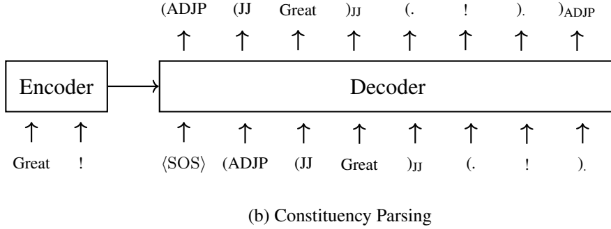
Figure 6.6: Illustration of tree linearization on either the encoder or the decoder side. For tree-to-string machine translation, the encoder takes a sequential representation of an input parse tree, and the decoder outputs the corresponding translation. For parsing, the encoder takes a sentence, and the decoder outputs the corresponding syntax tree.
