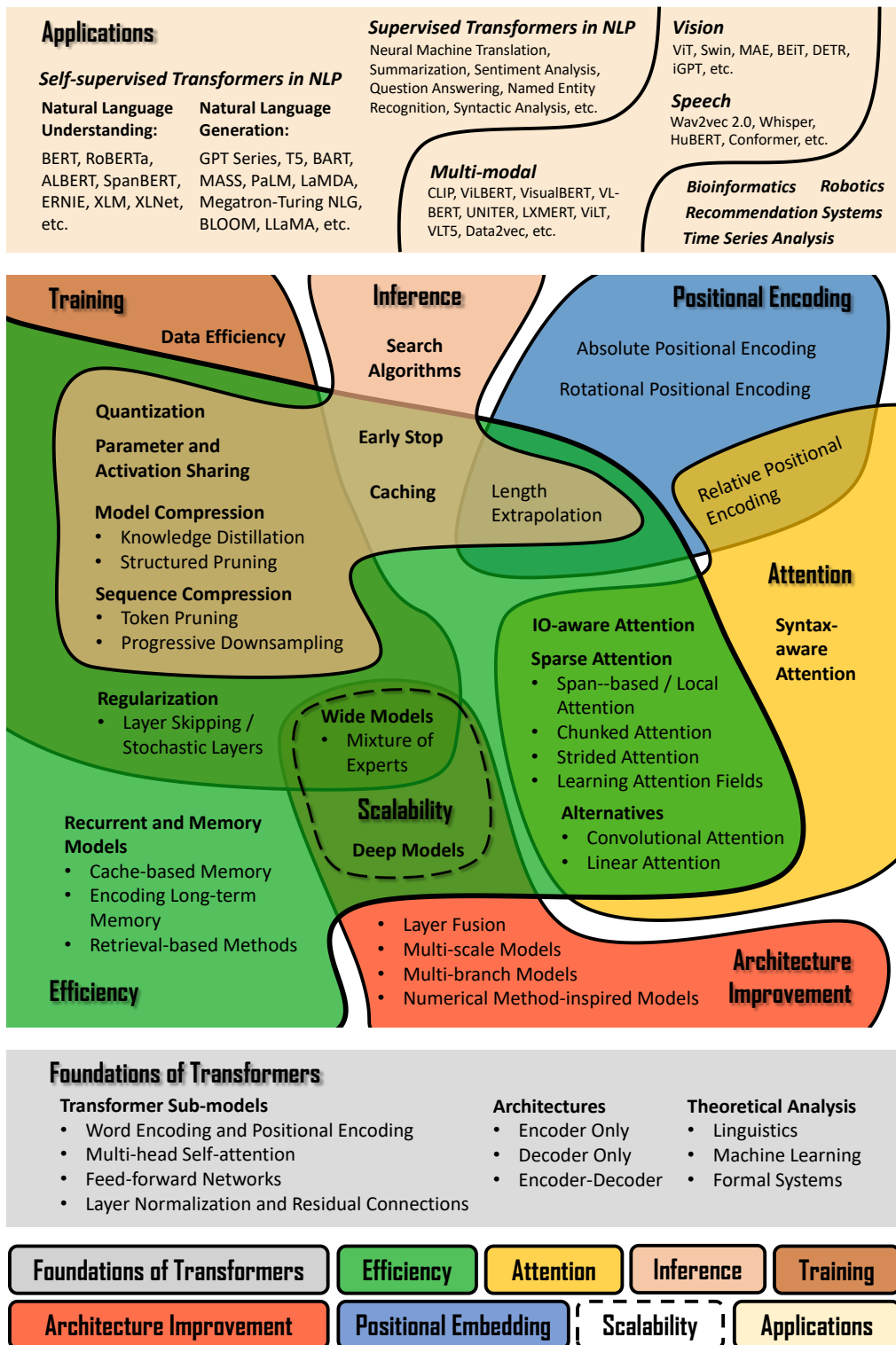
Figure 6.22: An overview of Transformers.
