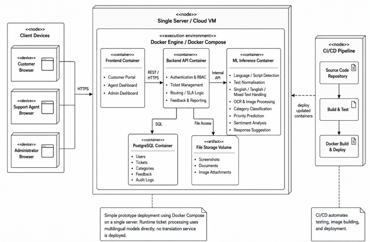
Deployment Diagram – Trilingual Customer Support Ticket Management System
