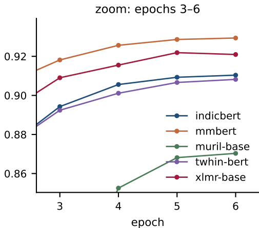
Intent macro-F1 by epoch — 4 of 5 models peak at the last epoch
