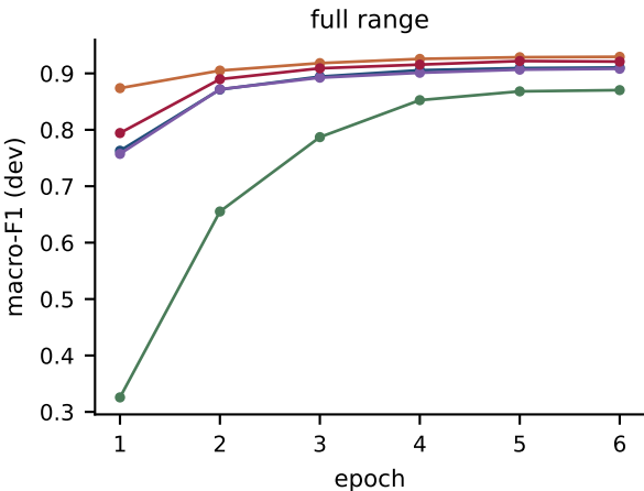
Intent macro-F1 by epoch — 4 of 5 models peak at the last epoch
