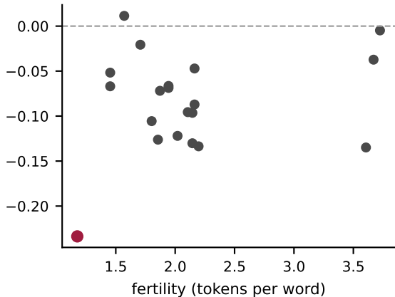
Characters lost to [UNK] predict the deficit; token count does not
