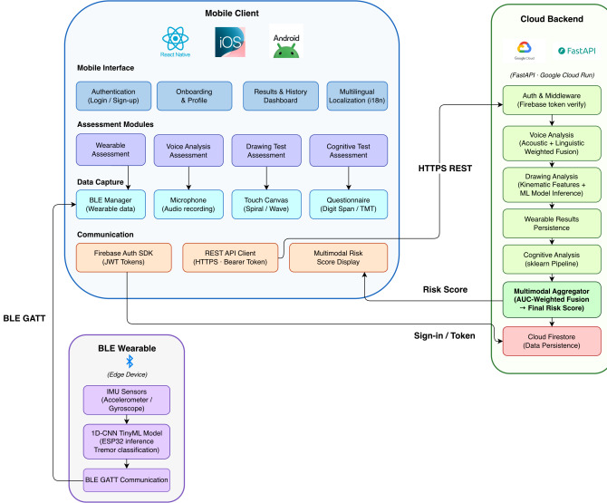
Figure 1 High Level Architecture Diagram
