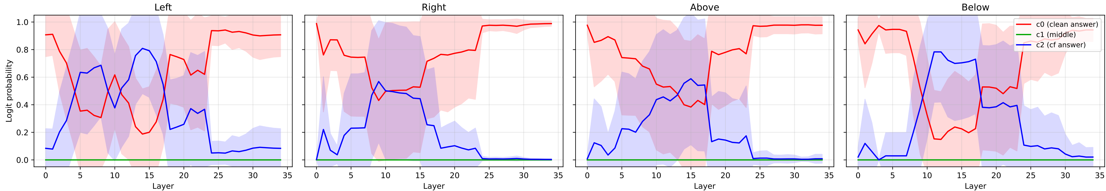
Object patching under ablation (Fig 9) — Squares · Gemma-3-4b-it (n=34)
