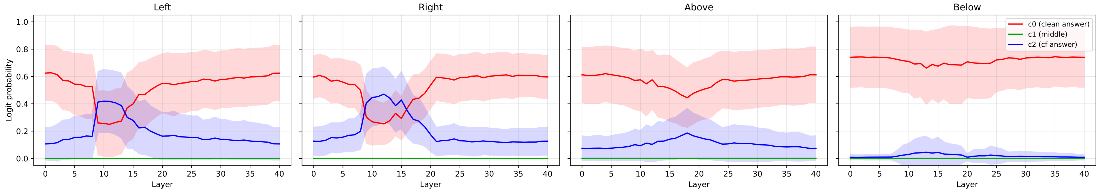
Object patching under ablation (Fig 9) — Objects · Pixtral-12B (n=36)
