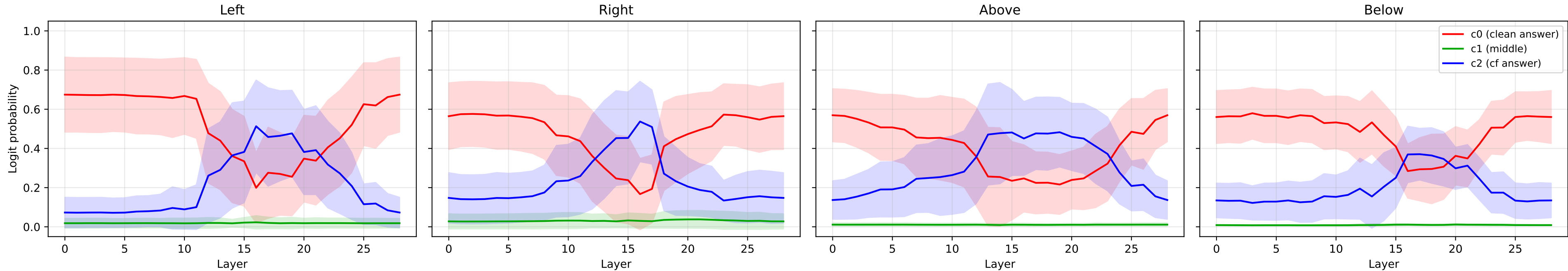
Object patching under ablation (Fig 9) — Shapes · Qwen2-VL-7B-Instruct (n=18)
