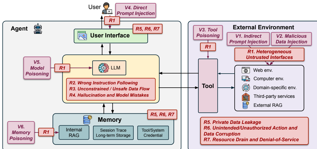
Figure 2: Demonstrations of attack vectors ( V^* ) and security risks ( R^* ) against agentic systems. Black boxes and arrows represent agent components and data flows. Purple boxes and arrows indicate attack vectors and how they enter the system. Red boxes indicate security risks.
