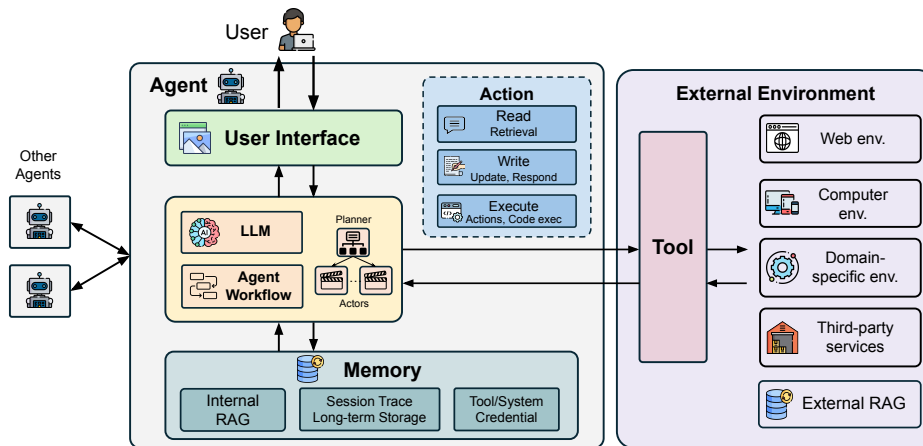
Figure 1: Overview of an AI Agent’s structure. The LLM and agent workflow together govern the agent’s planning and execution. Multi-agent systems have multiple such cores, each with their own memory, system prompts, and tool sets.
