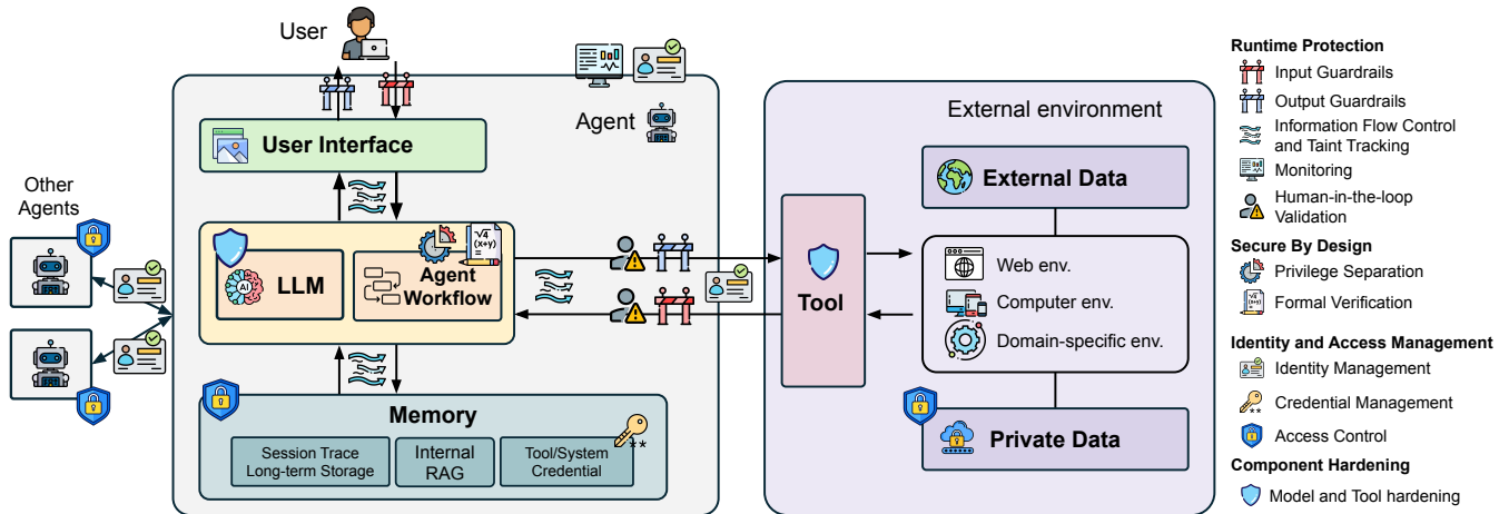
Figure 4: The defense landscape of AI agents, showing which components or stages of the control flow each defense targets.
