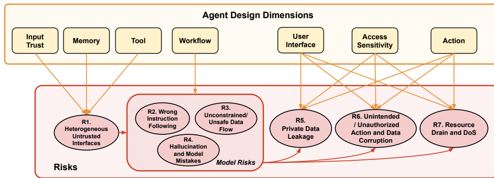
Figure 3: Relationship between agent design dimension and risks, and the connection across different risks.
