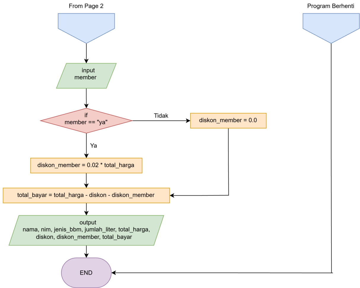
Gambar 1.3 Flowchart
