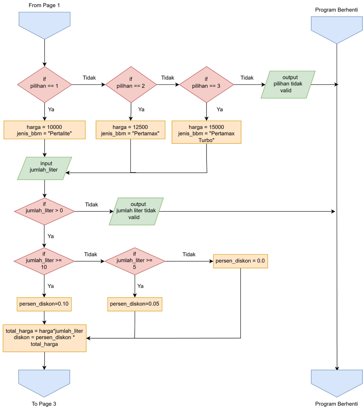
Gambar 1.2 Flowchart
