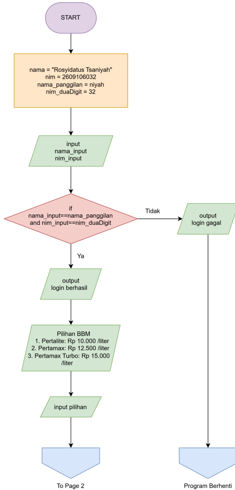
Gambar 1.1 Flowchart
