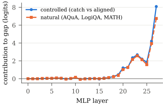
(b) Same late MLPs carry the gap
