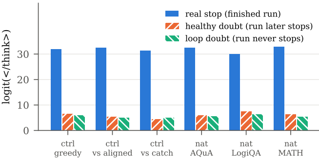
(a) The stop gate opens only at the real stop
