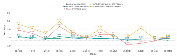
Figure 7: Dyck accuracy.
