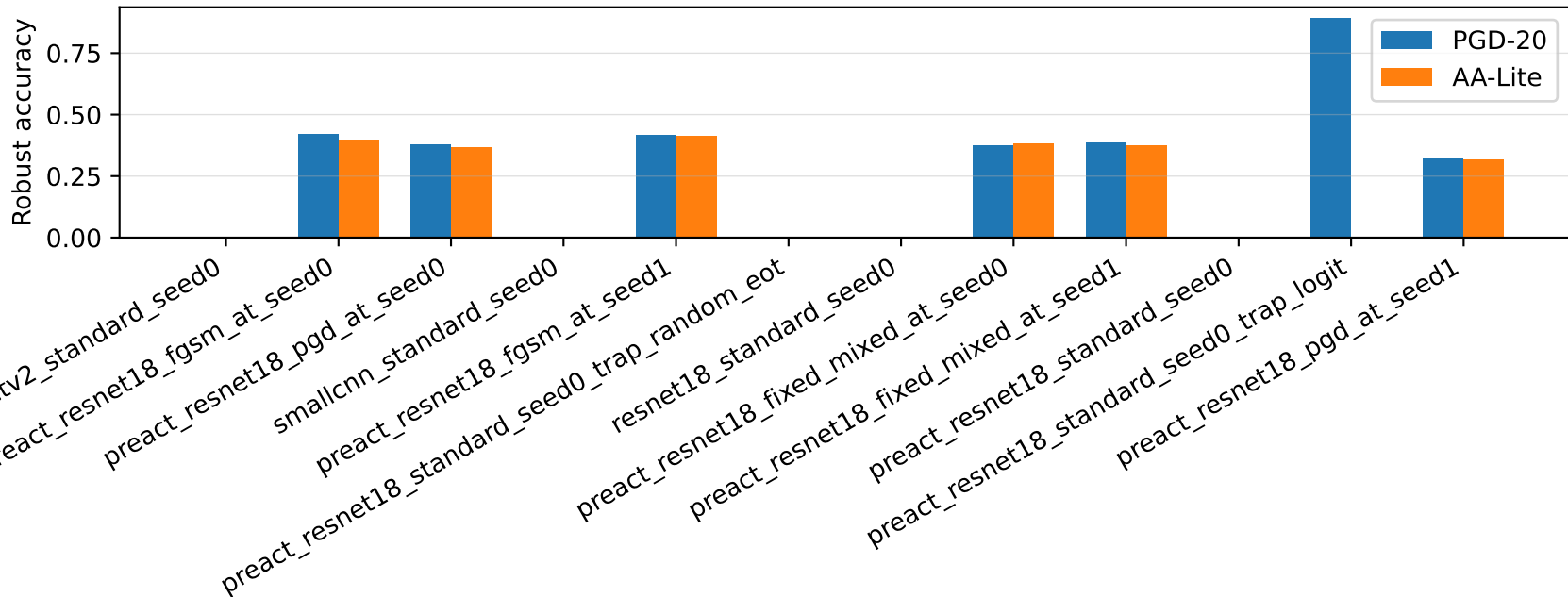
PGD-only vs AA-Lite
