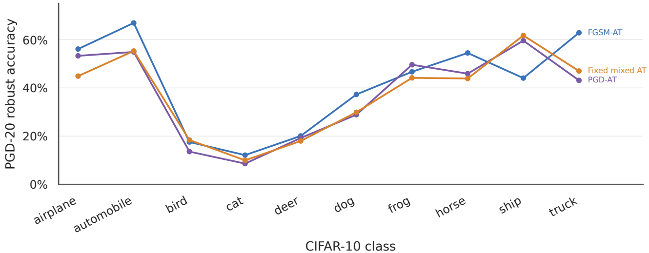
Class-level PGD-20 robustness remains uneven across adversarial-training recipes
