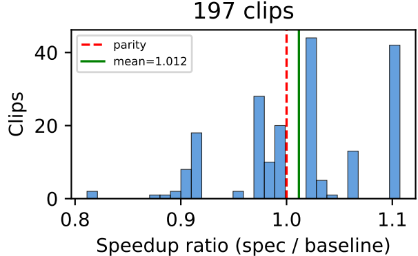
Figure 3: Per-clip speedup ratio (speculative / baseline) over 197 paired clips. The mean is 1.012\times ; speculation is faster on 53.3% of clips.
