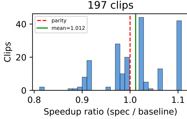
Figure 3: Per-clip speedup ratio (speculative / baseline) over 197 paired clips. The mean is 1.012 \times ; speculation is faster on 53.3% of clips.
